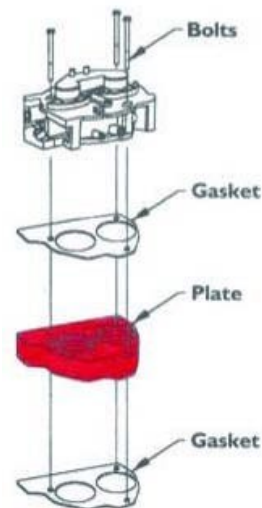
Throttle Body Showing Bolts, Gaskets, and Plate
